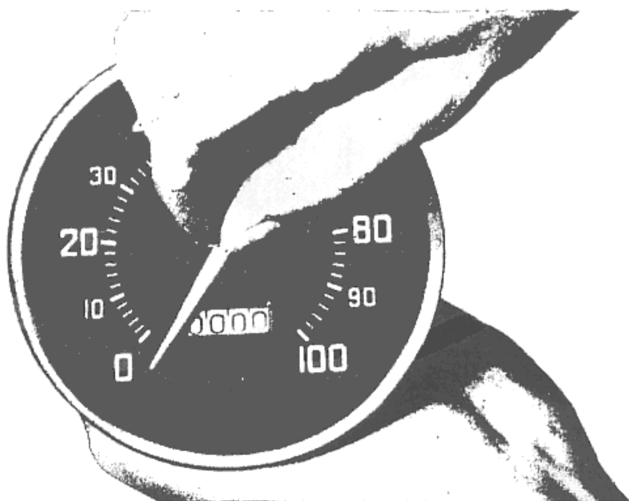
Figure 77—Driving Off Pressed-on Bezel, Using Remover (T-42358)
