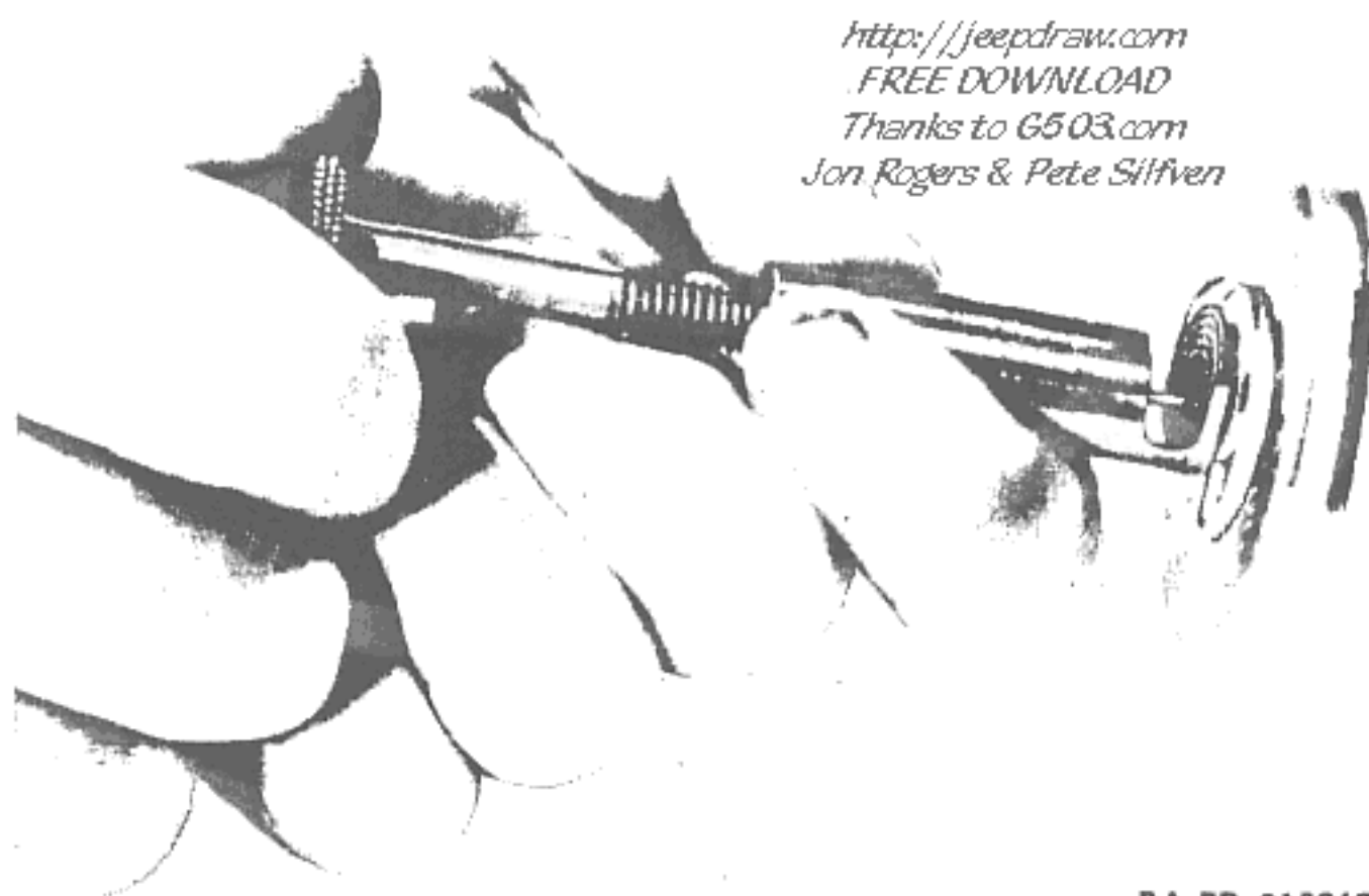
Figure 84—Removing Hair Spring, Using Puller (T-66296)
