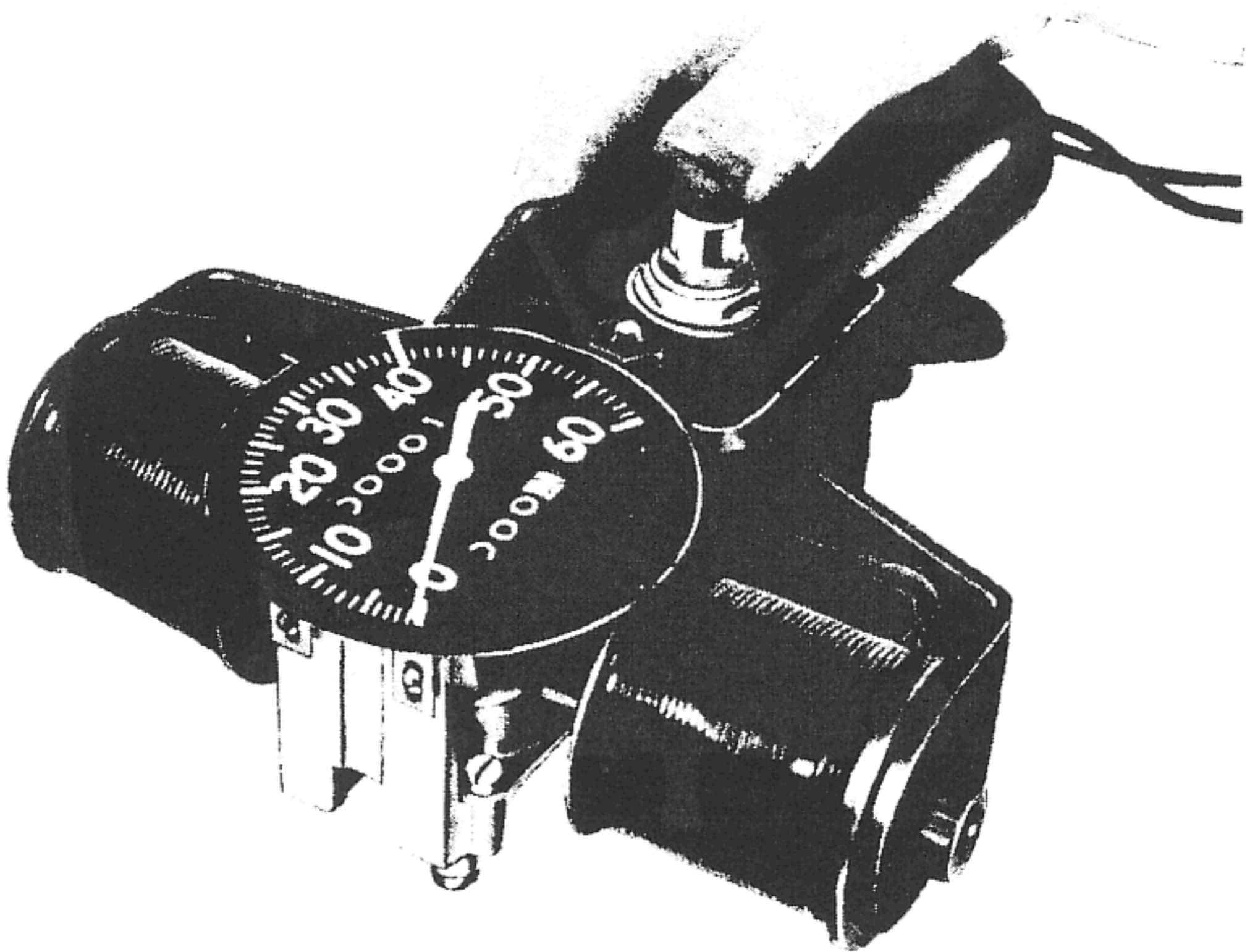
Figure 23—Charging AC Speedometer or Tachometer Magnet, Using Magnetizer (846294)
