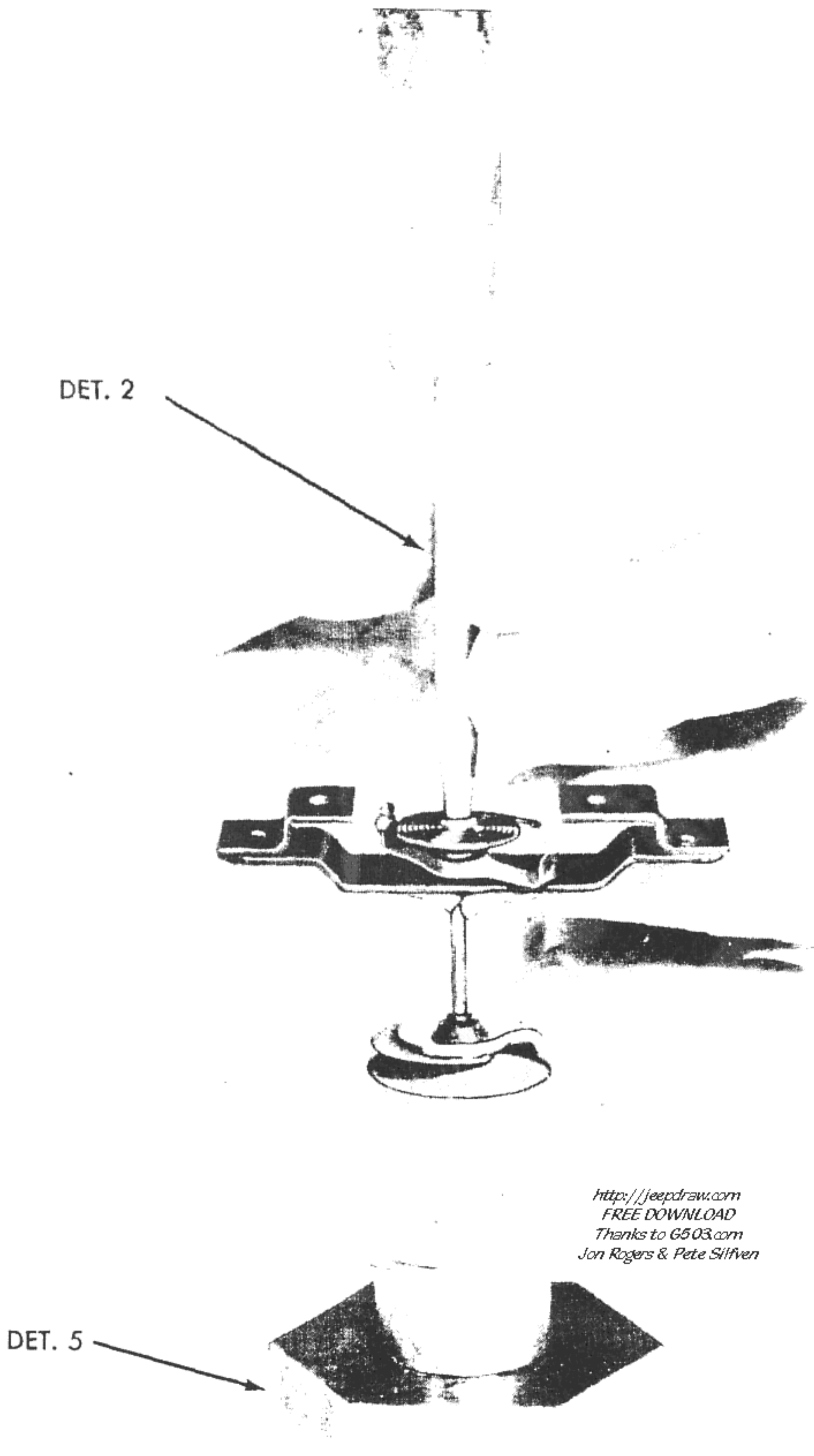
Figure 70—Replacing Hair Spring, Using Assembly Kit (T-29)
