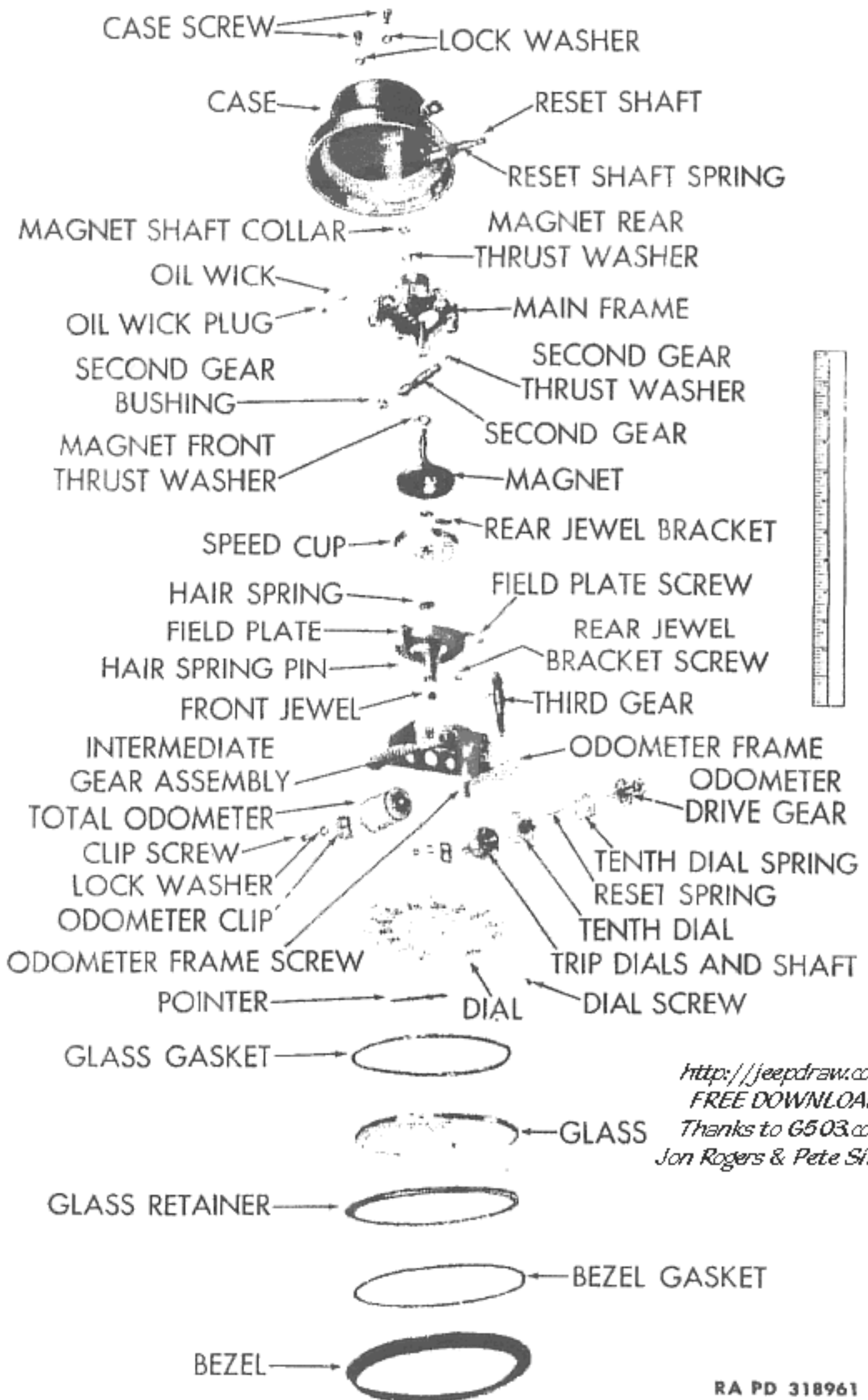
Figure 76—Stewart-Warner Speedometer with Flat Disk-type Magnet Disassembled
