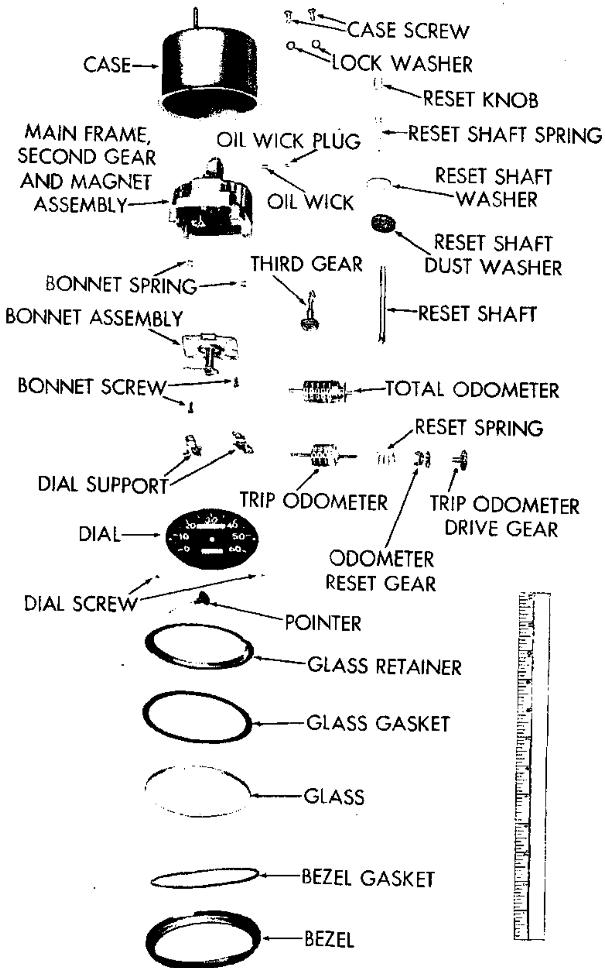
Figure 113—Waltham Speedometer, Disassembled
