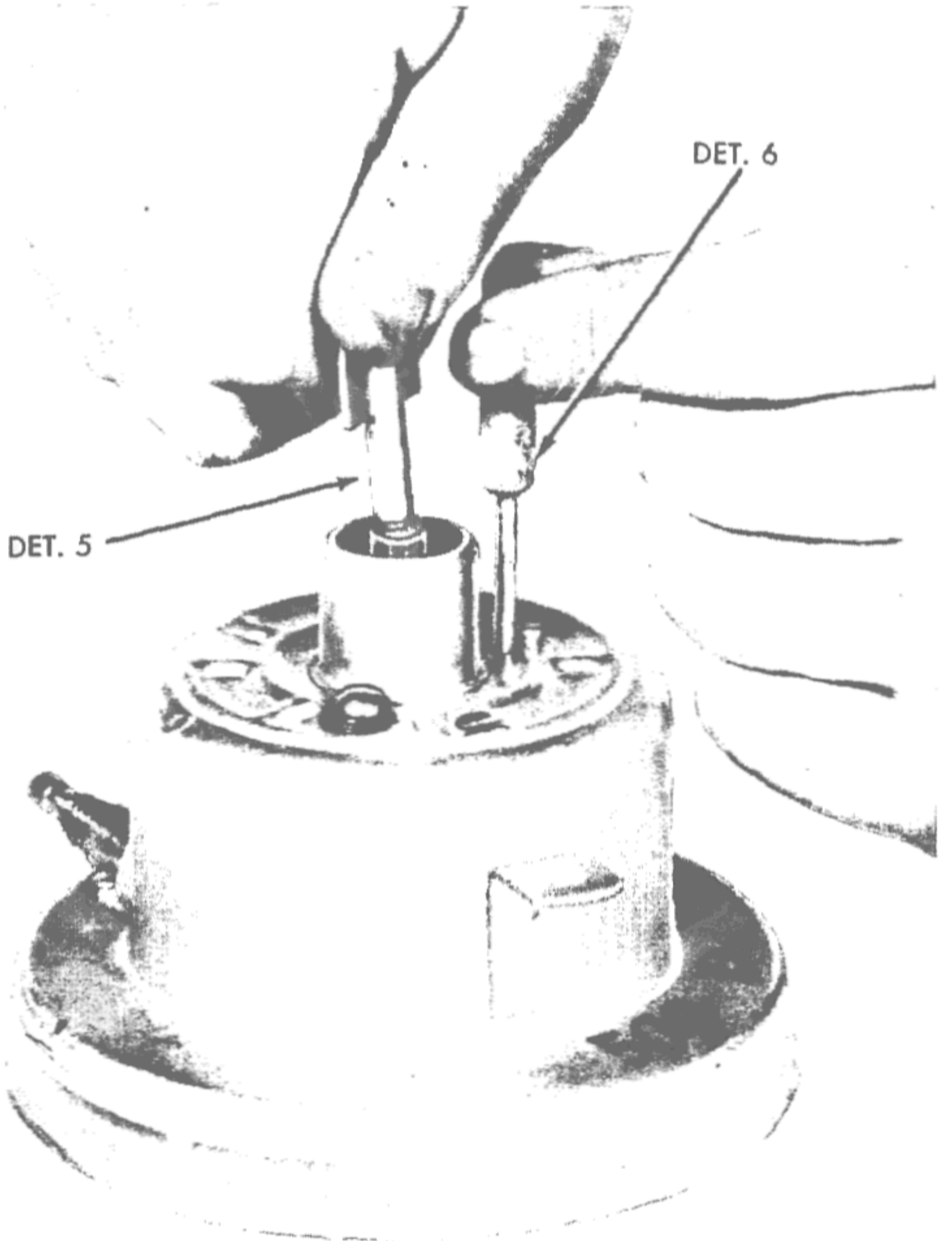
Figure 102—Moving Magnet Regulator, Using Adjusting Kit (T-178715)
