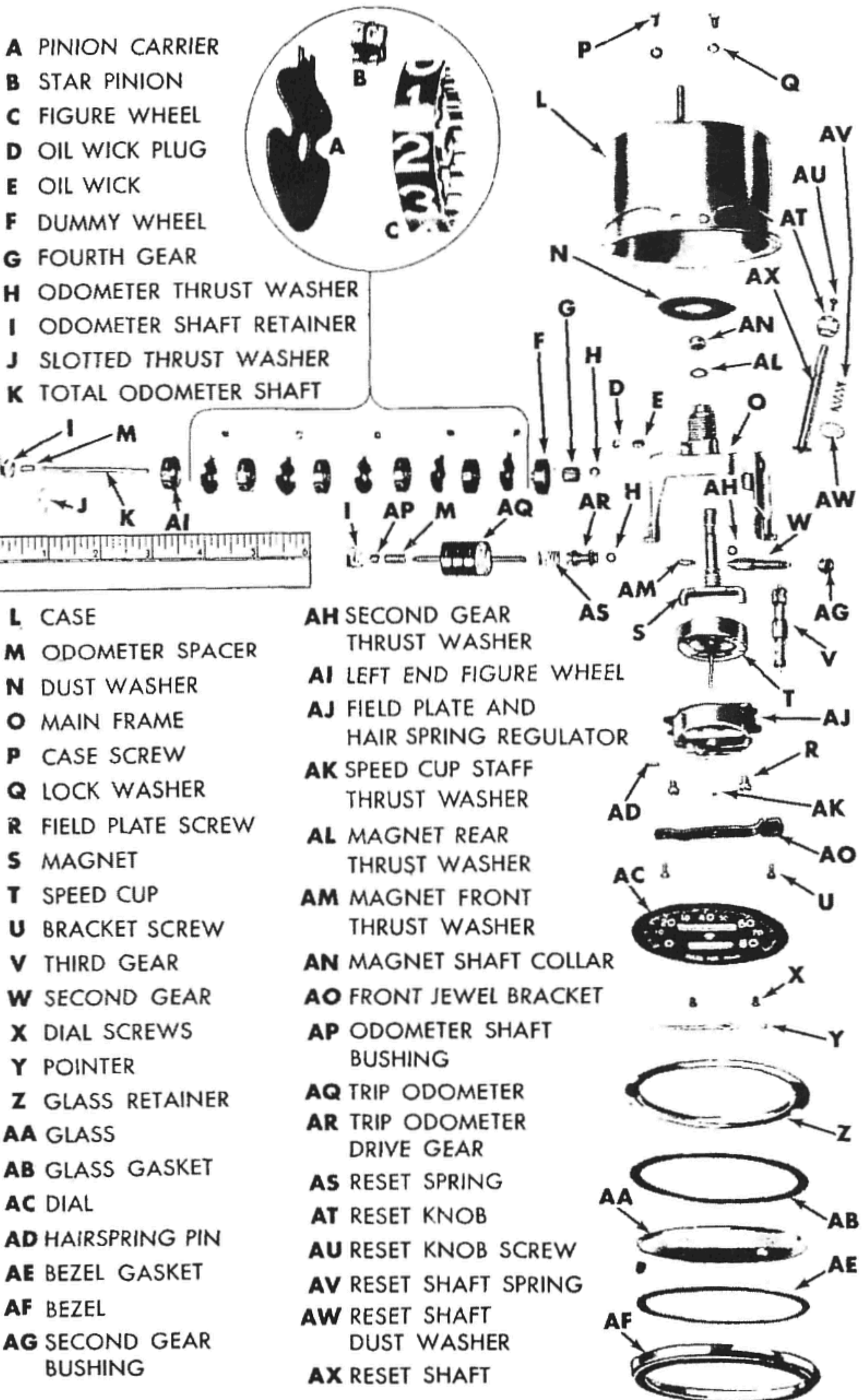
Figure 15—AC Speedometer Disassembled
