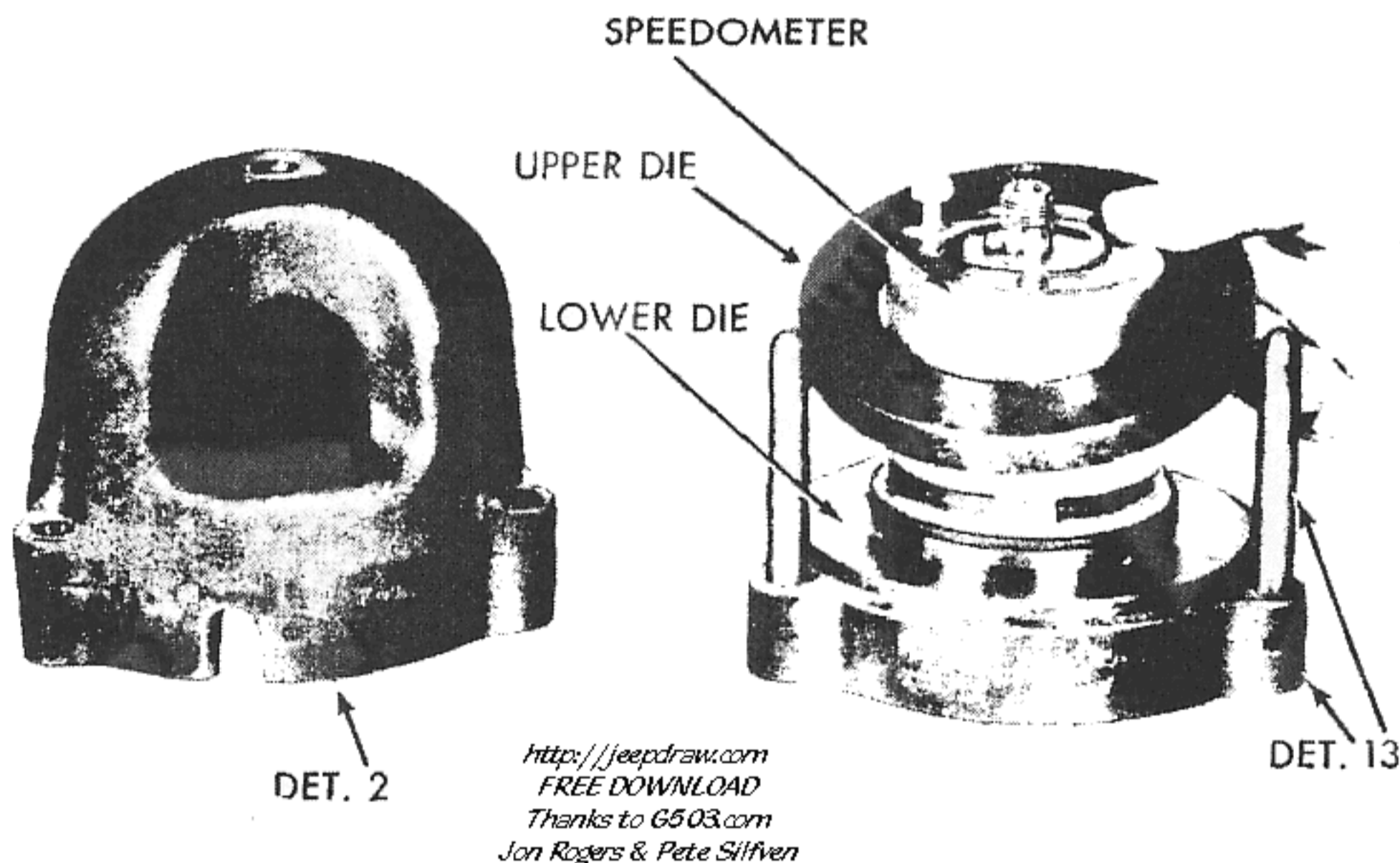
Figure 74—Placing Upper Die of Bezel Rolling Fixture (T-178730) Over Speedometer
