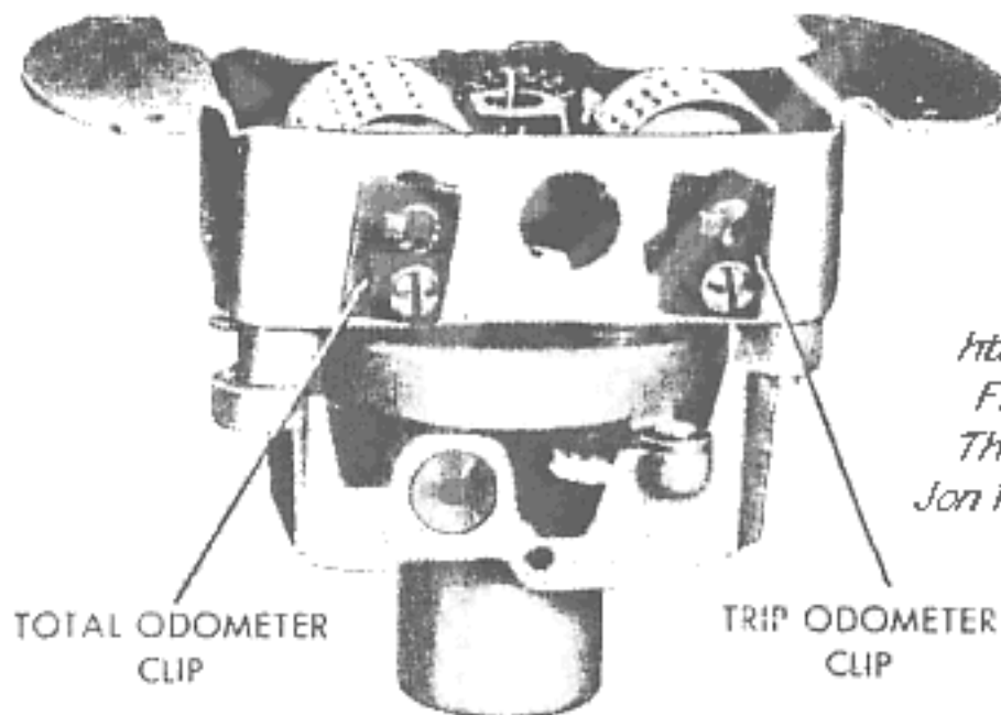
Figure 81—Speedometer Mechanism (Dial Removed)
