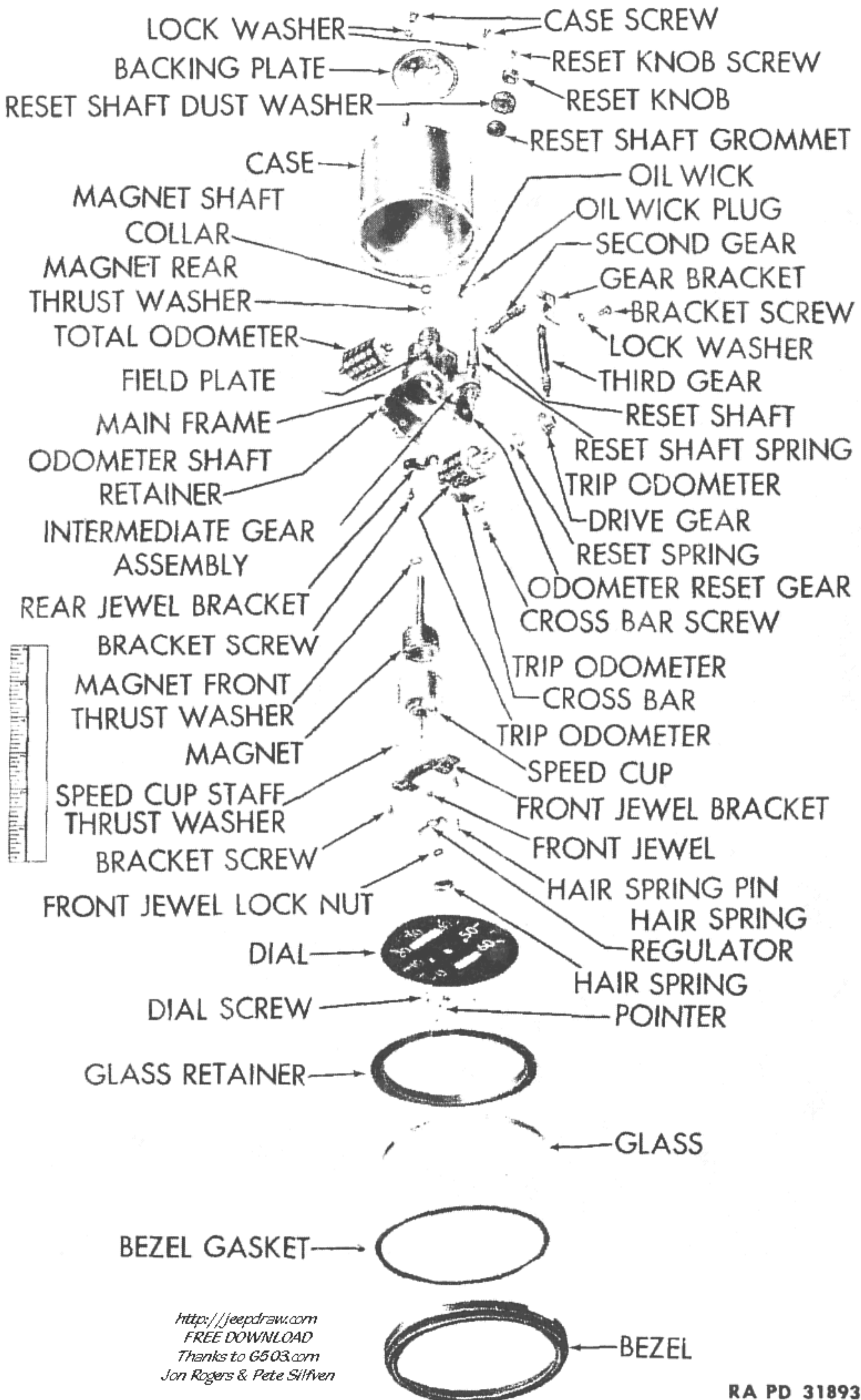
Figure 50—Stewart-Warner Speedometer with Cup-type Magnet Disassembled
