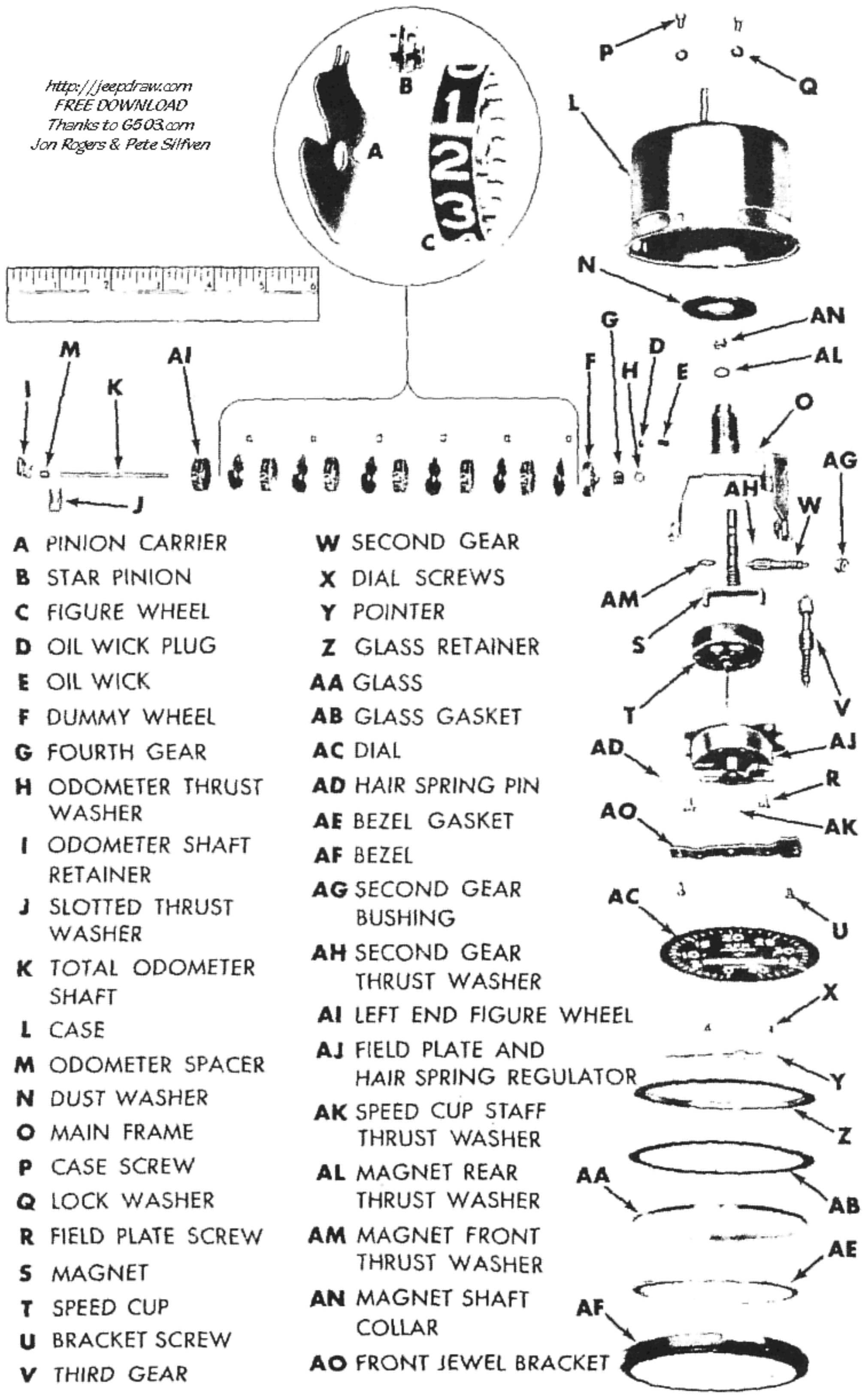
Figure 16—AC Tachometer Disassembled
