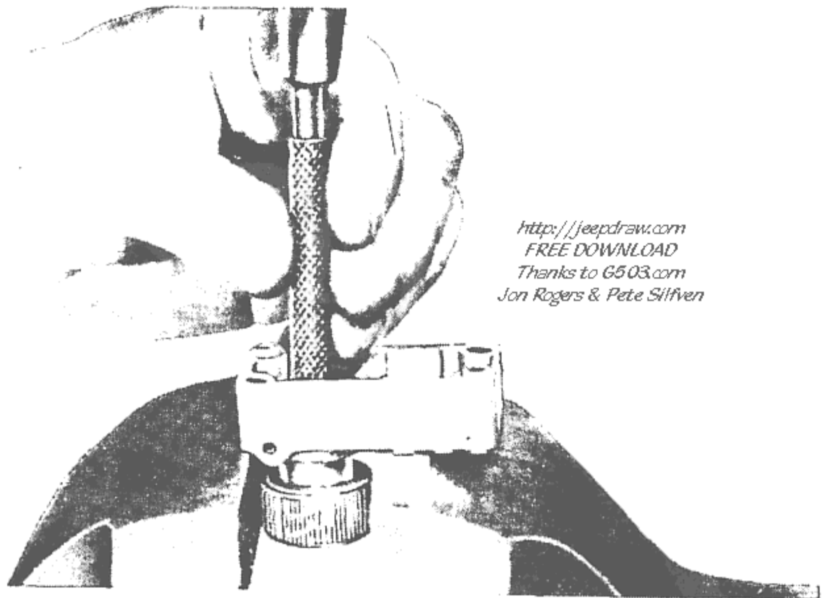
Figure 140—Driving Out Sleeve
