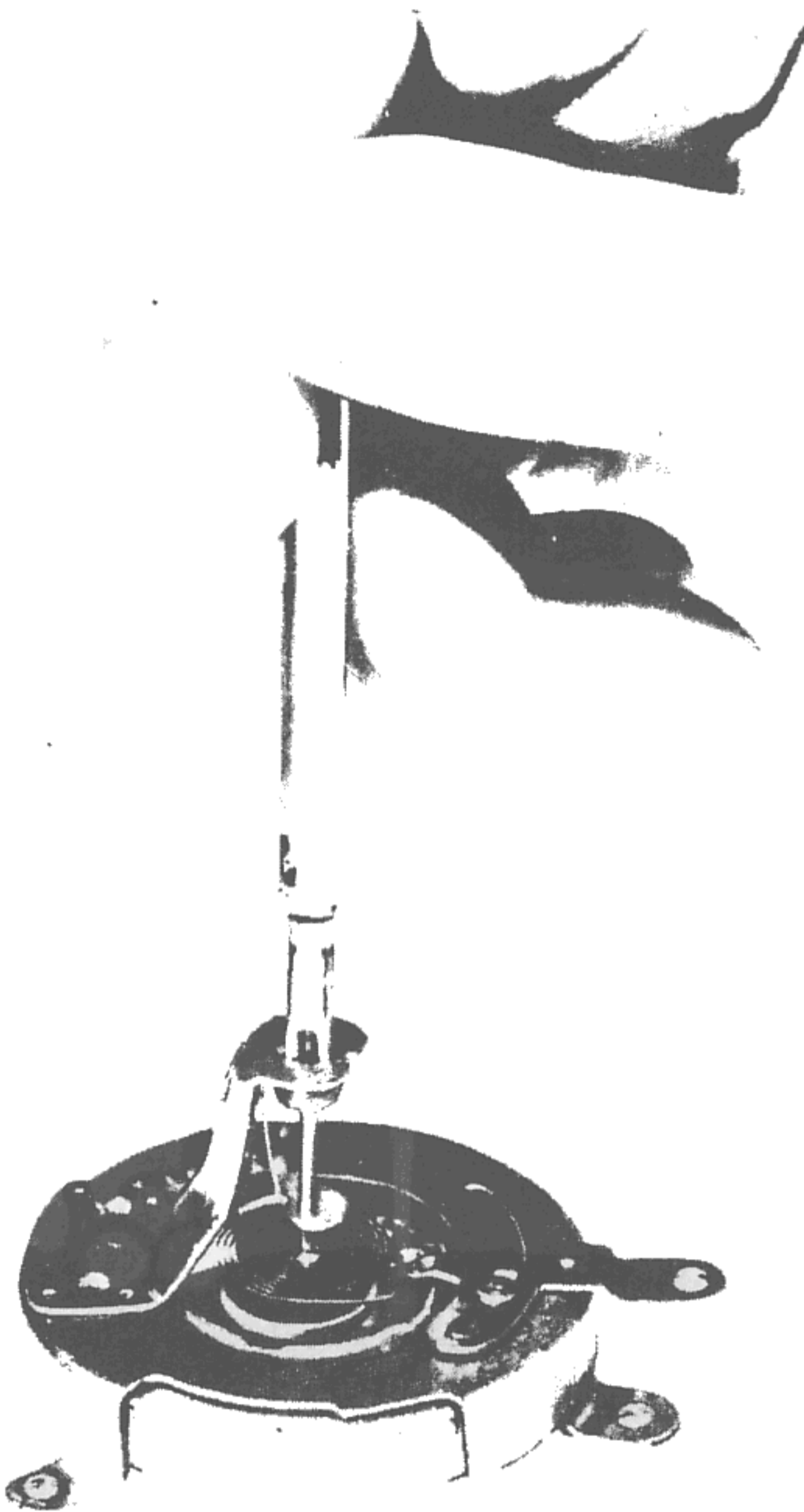
Figure 96—Adjusting Front Jewel, Using Special Tool (T-178705)
