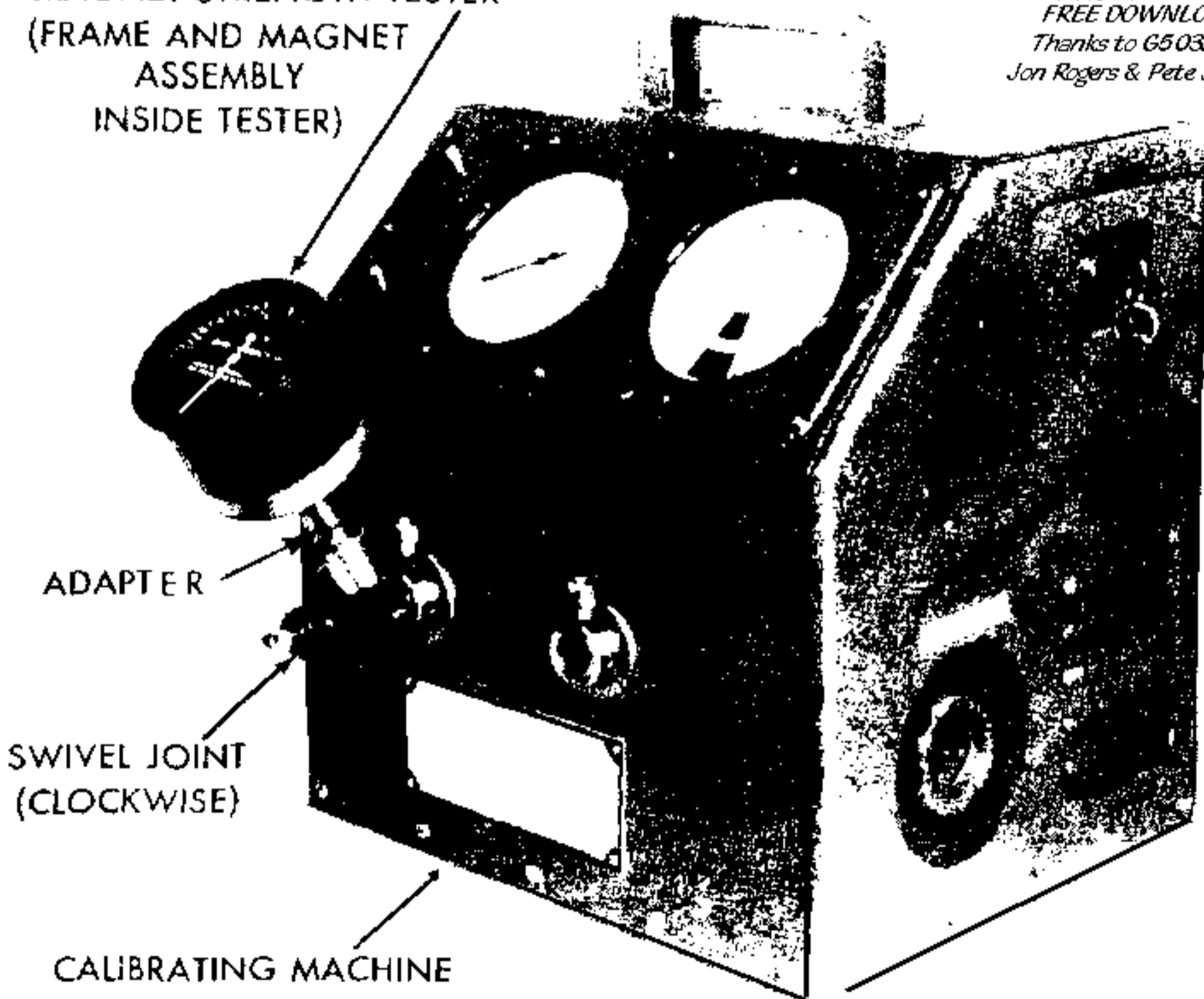
Figure 69—Magnet Strength Tester (408165) (on Frame and Magnet Assembly) Attached to Calibrating Machine (T-170645)
