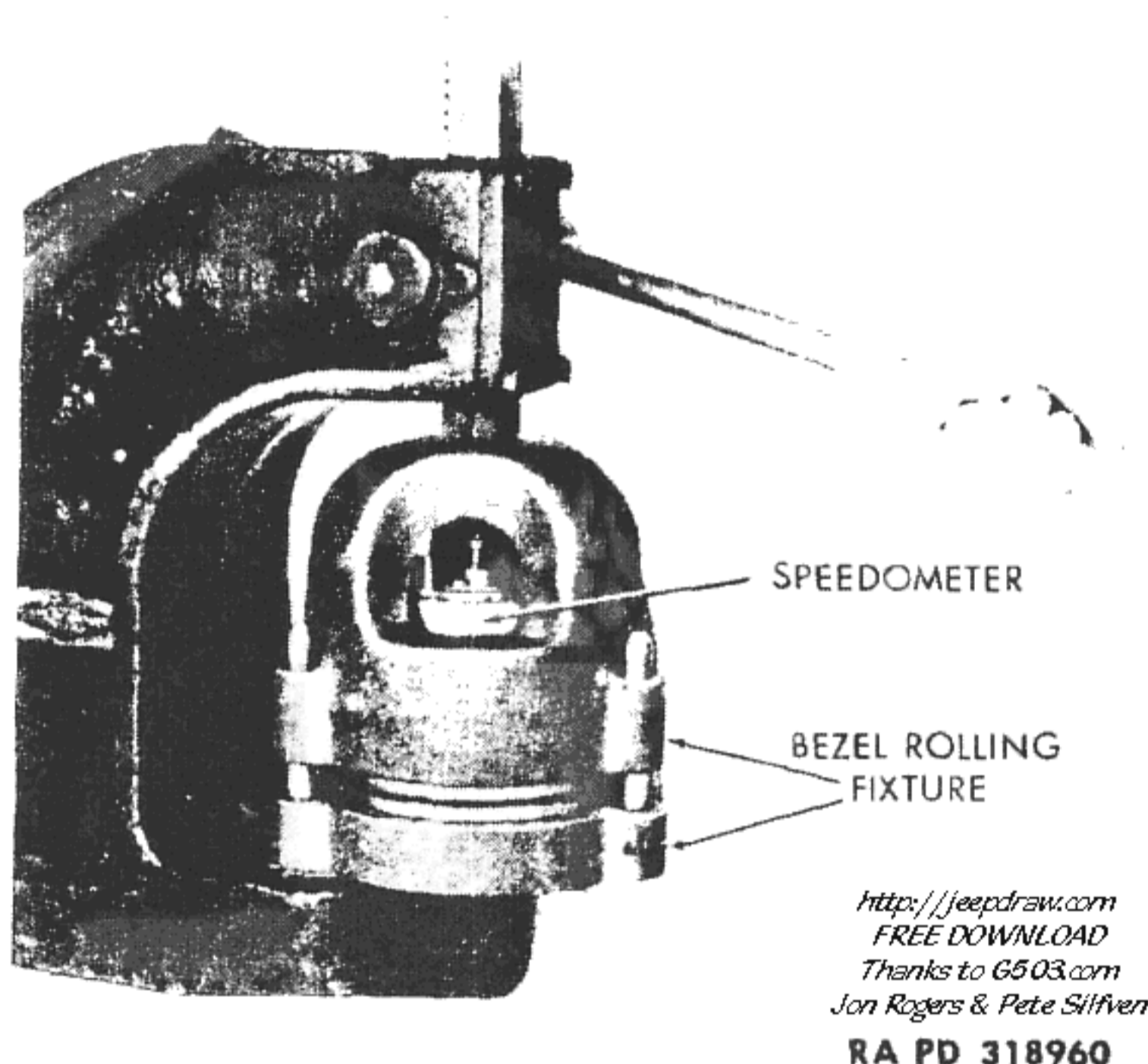
Figure 75—Rolling Bezel with Fixture (T-178730) in Arbor Press
