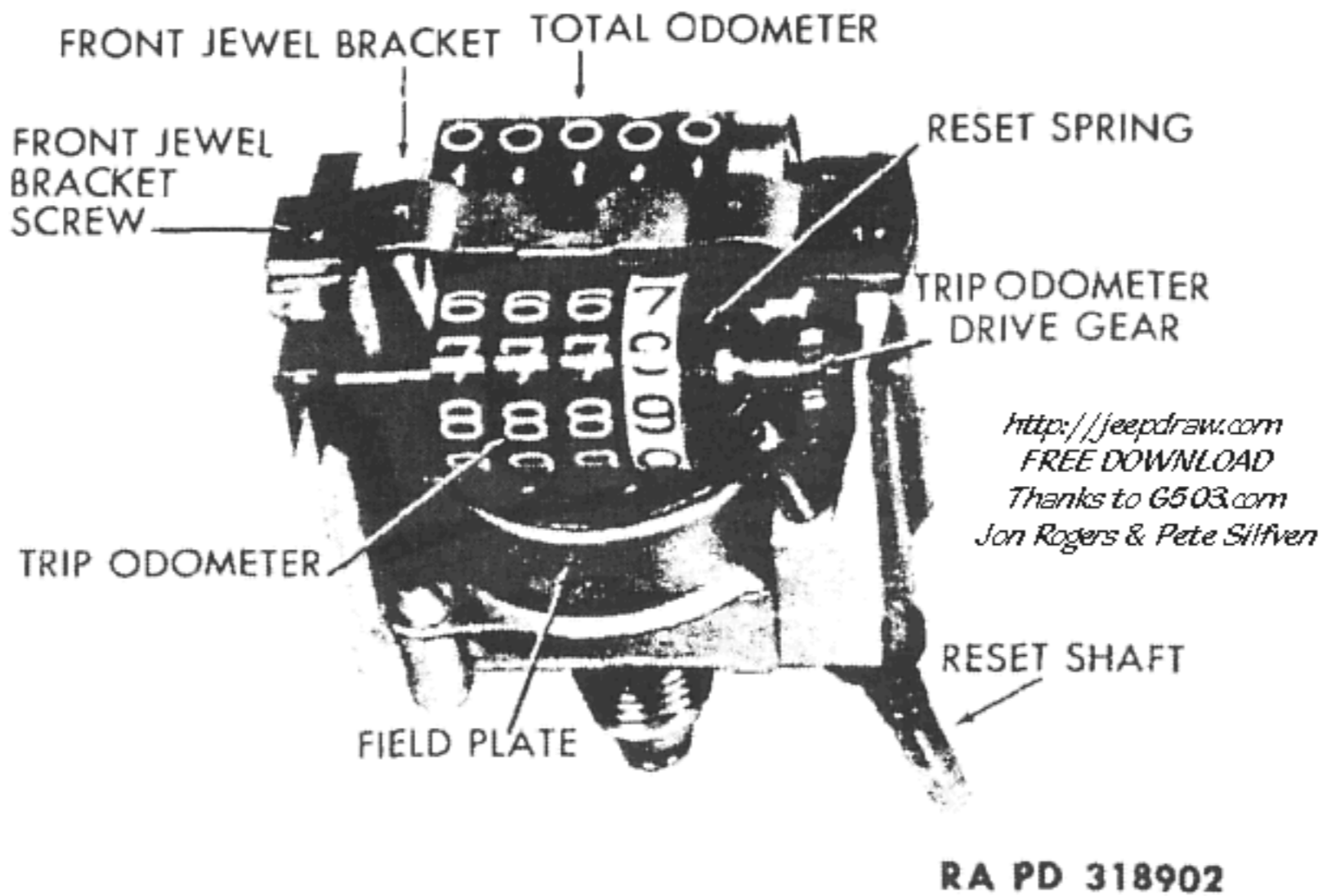
Figure 17—Speedometer Mechanism (Dial Removed)
