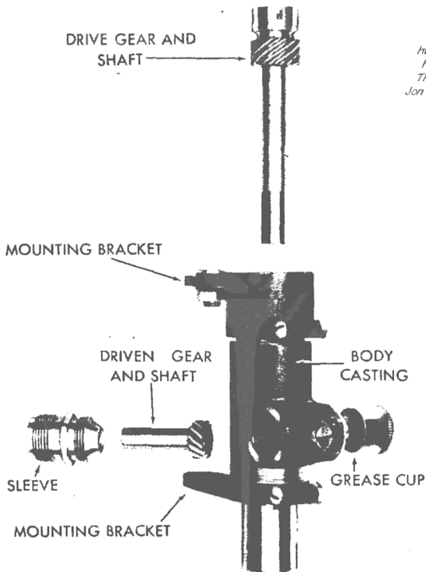
Figure 150—Stewart-Warner 659-type Drive Joint, Partially Disassembled
