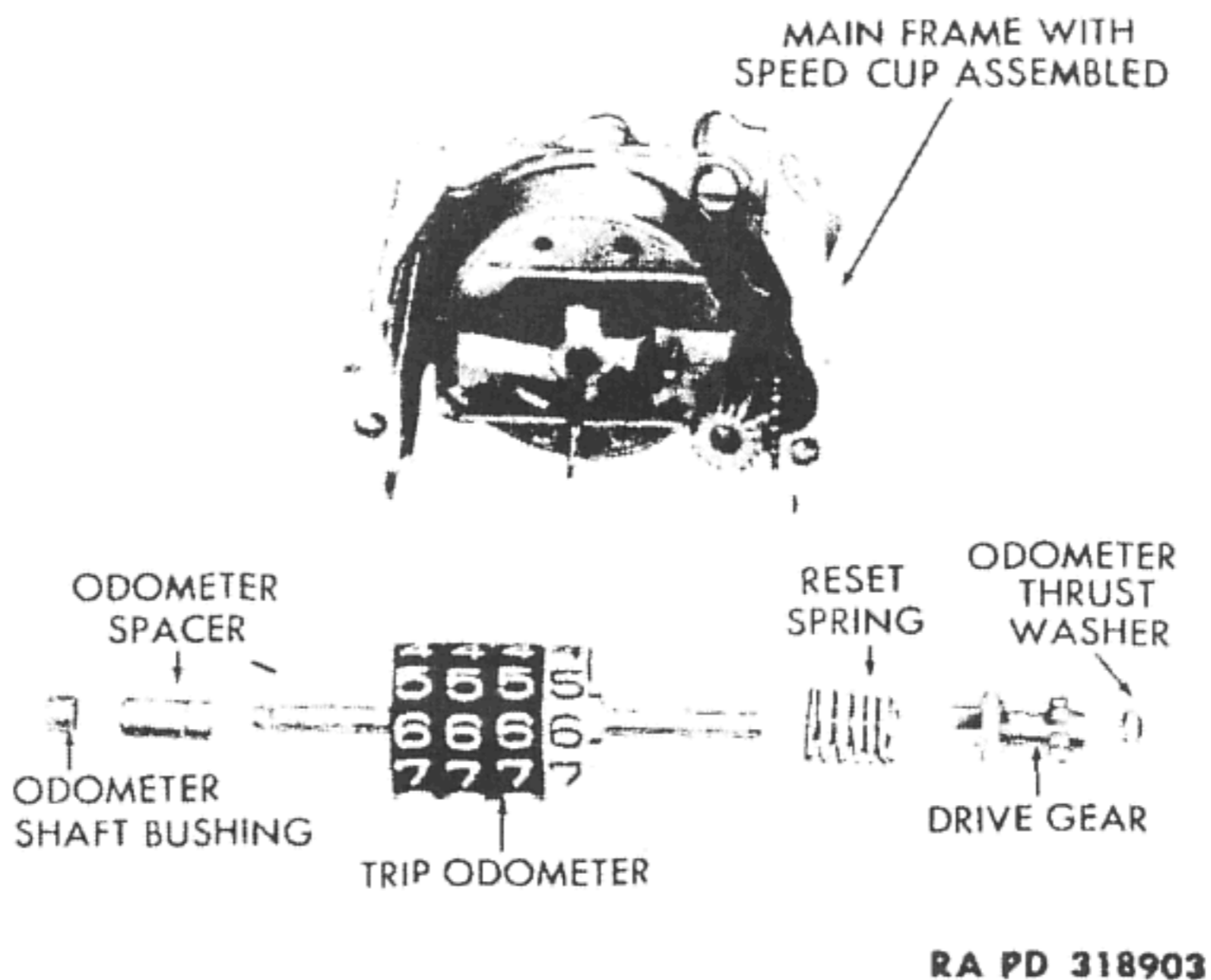
Figure 18—Quick Reset Trip Odometer Removed from Frame
