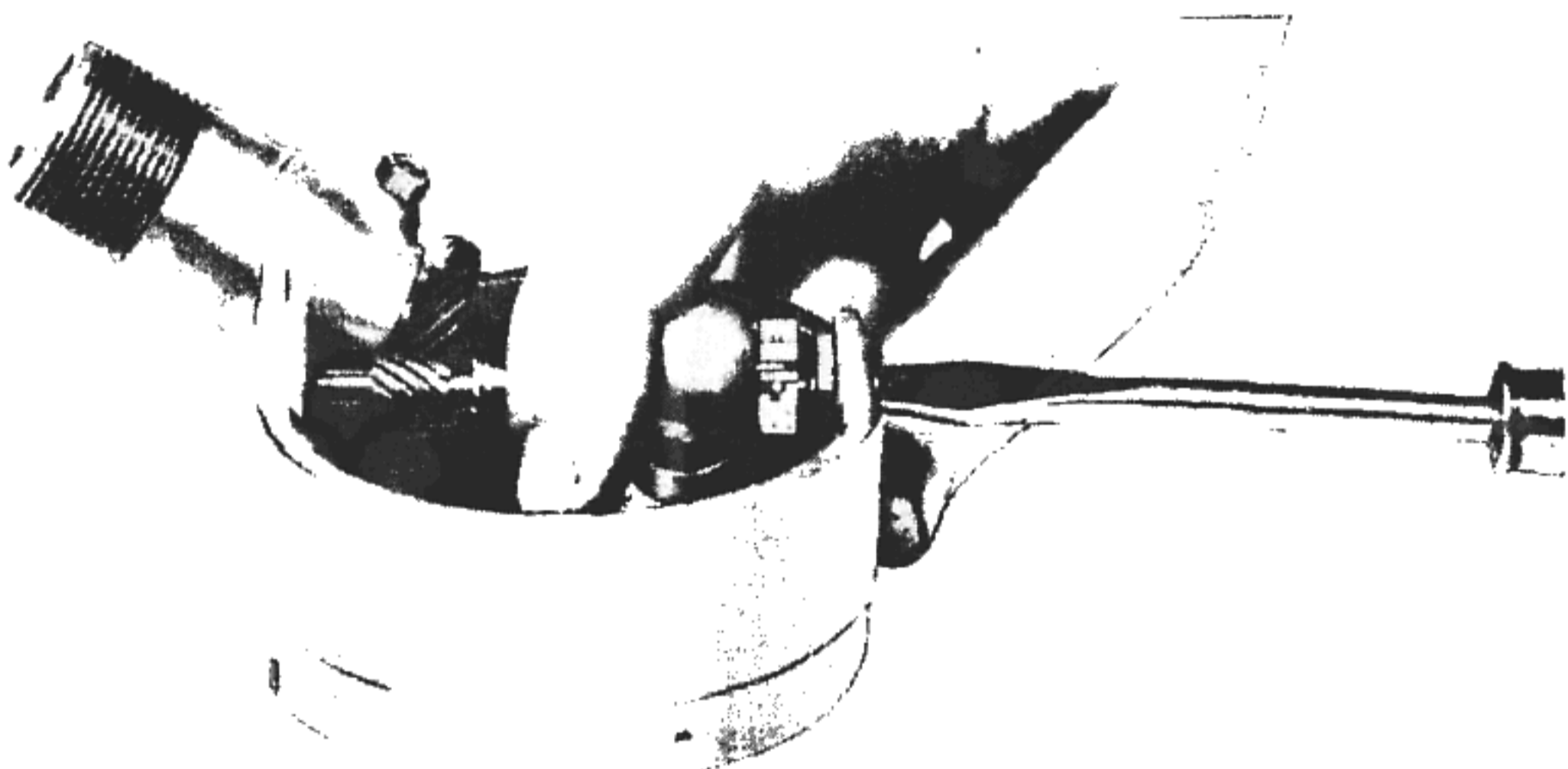
Figure 109—Unscrewing Upper Ball Race
