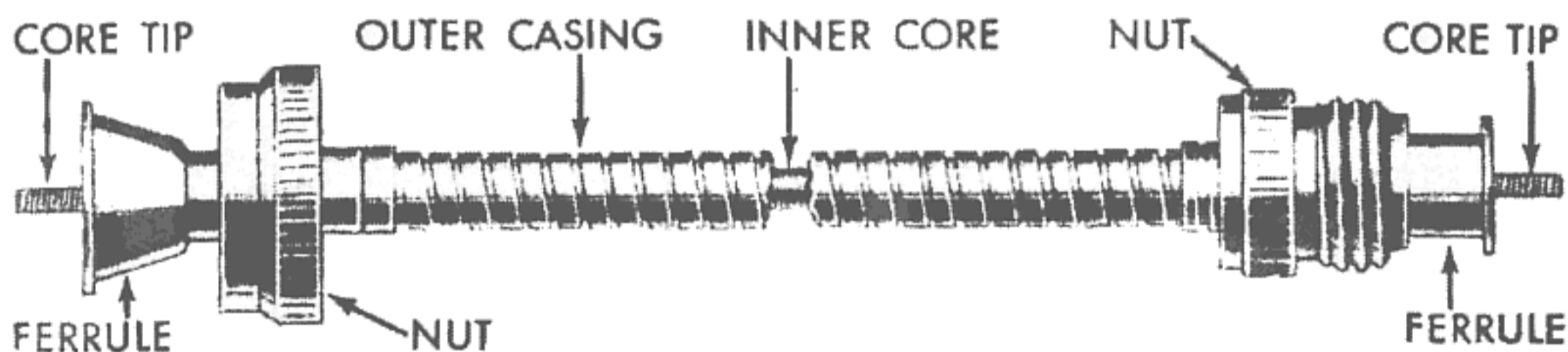
Figure 124—Flexible Shaft
