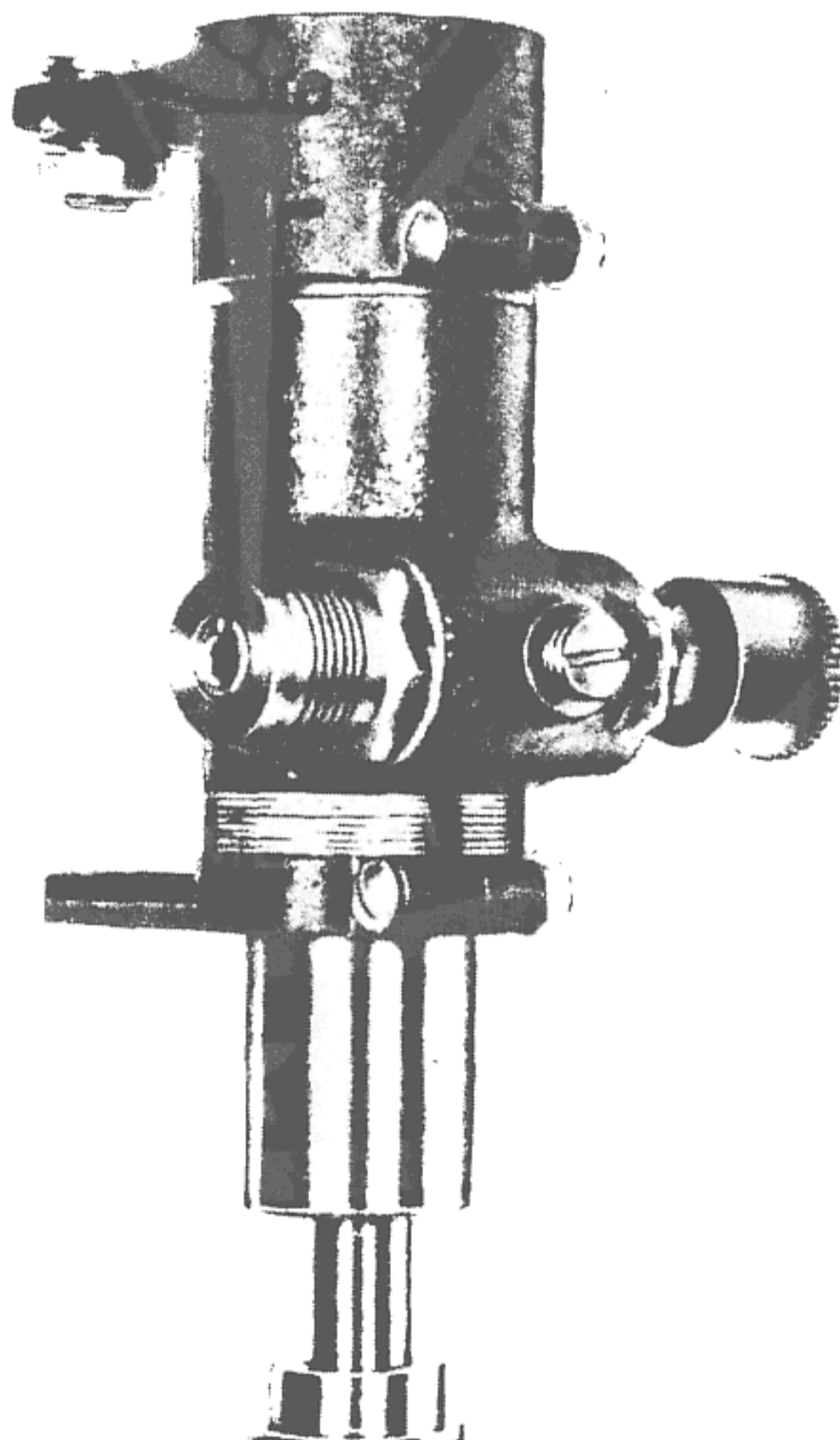
Figure 149—Stewart-Warner 659 Distributor-type Drive Joint
