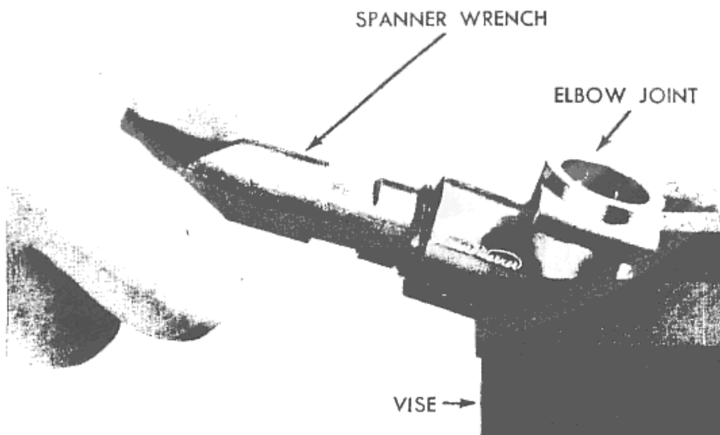
Figure 80—Removing Bevel Gear and Sleeve Assembly, Using Spanner Wrench (T-49509)
