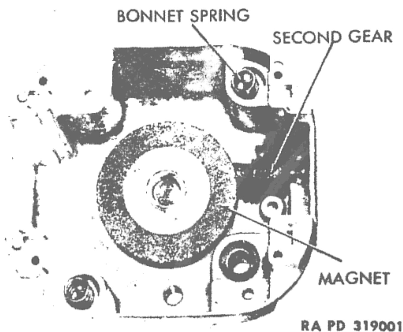
Figure 116—Frame, Second Gear, and Magnet Assembly
