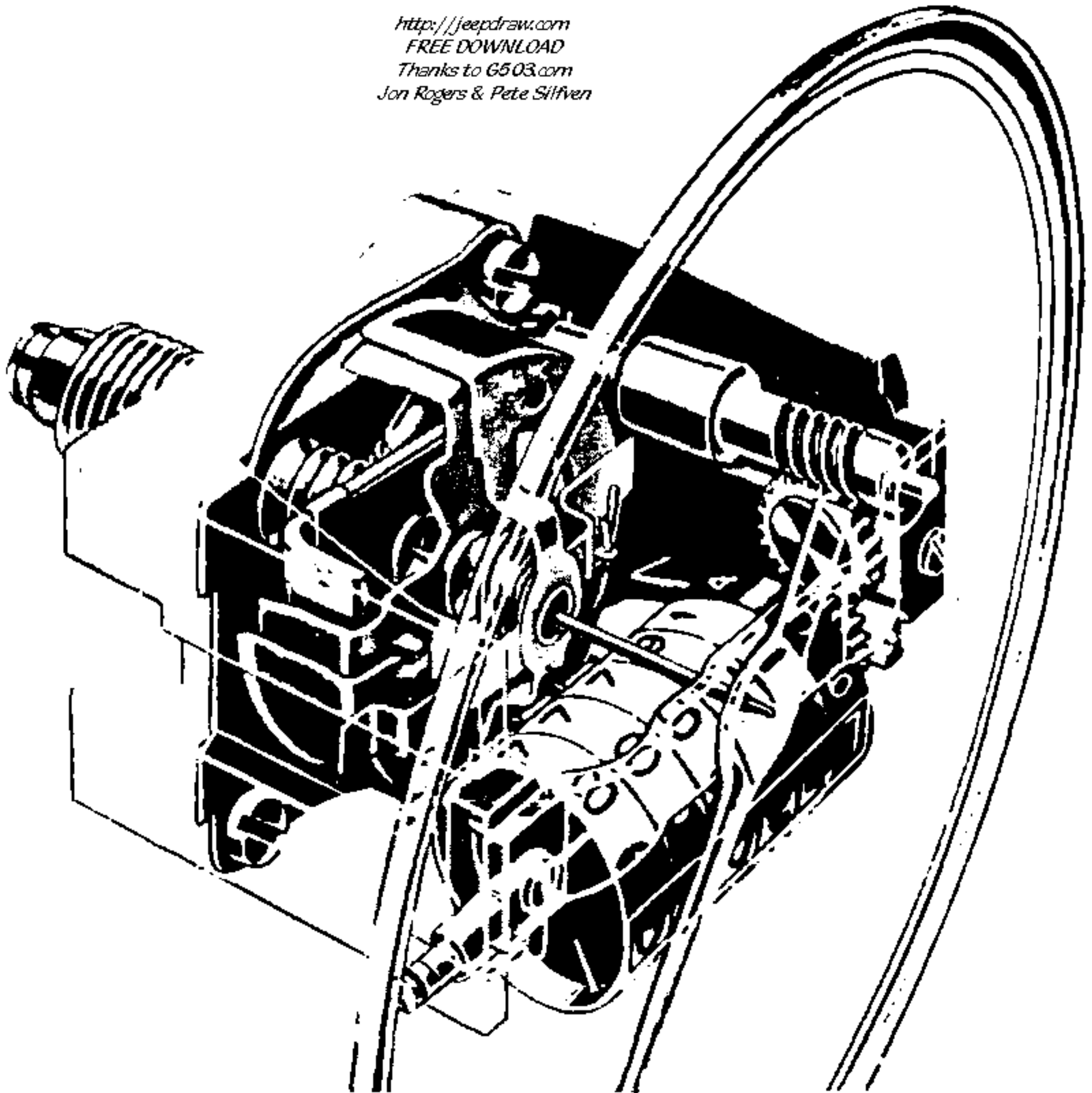
Figure 6—Phantom View of Speedometer
