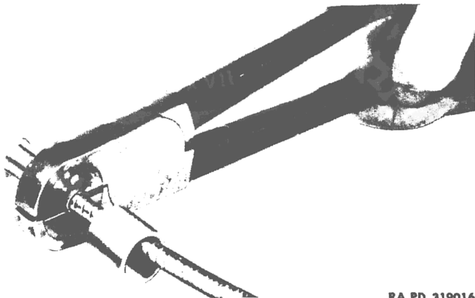
Figure 131—Crimping Ferrule, Using Pliers (T-122308)
