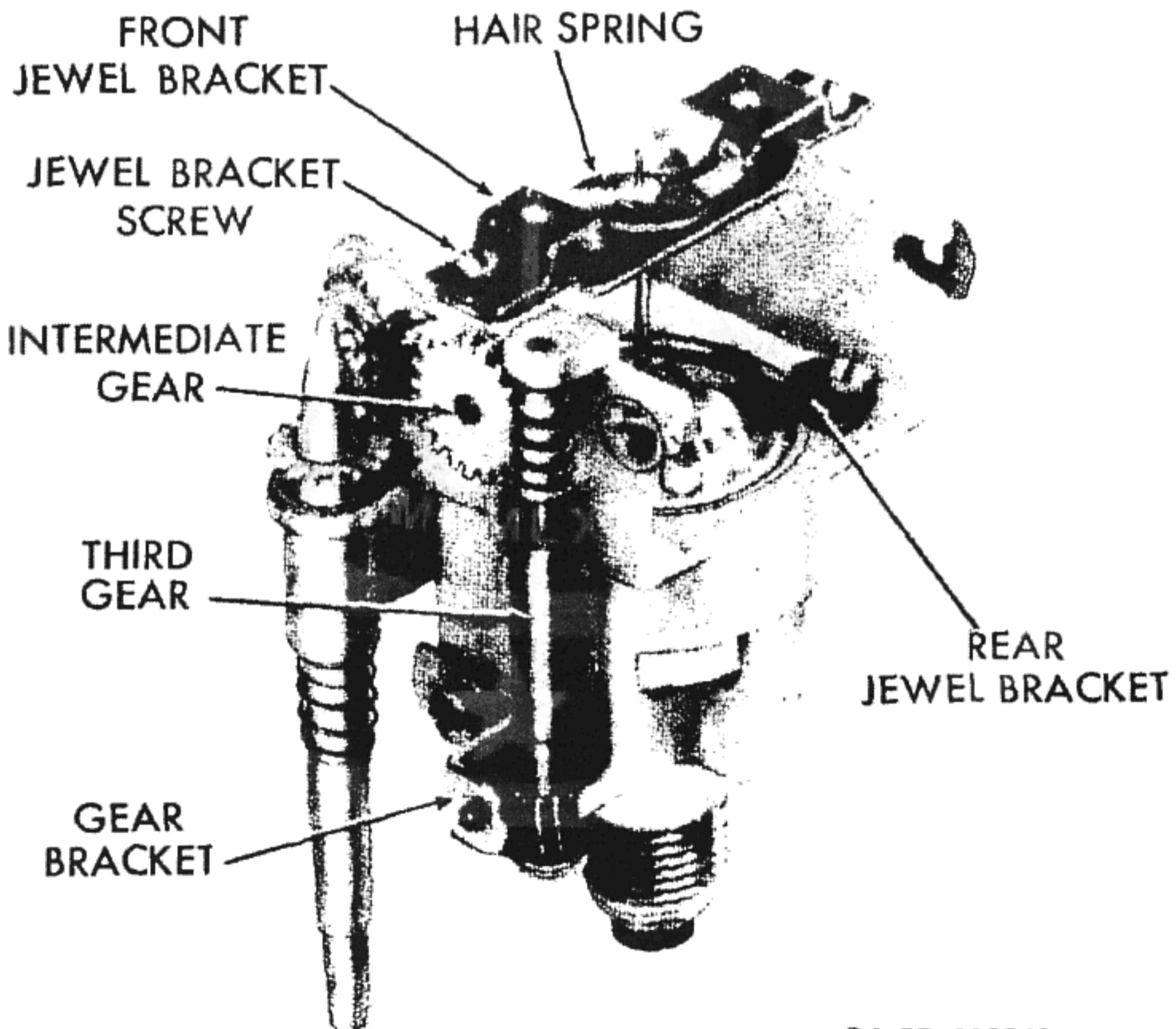
Figure 56—Speedometer Mechanism (Odometers Removed)
