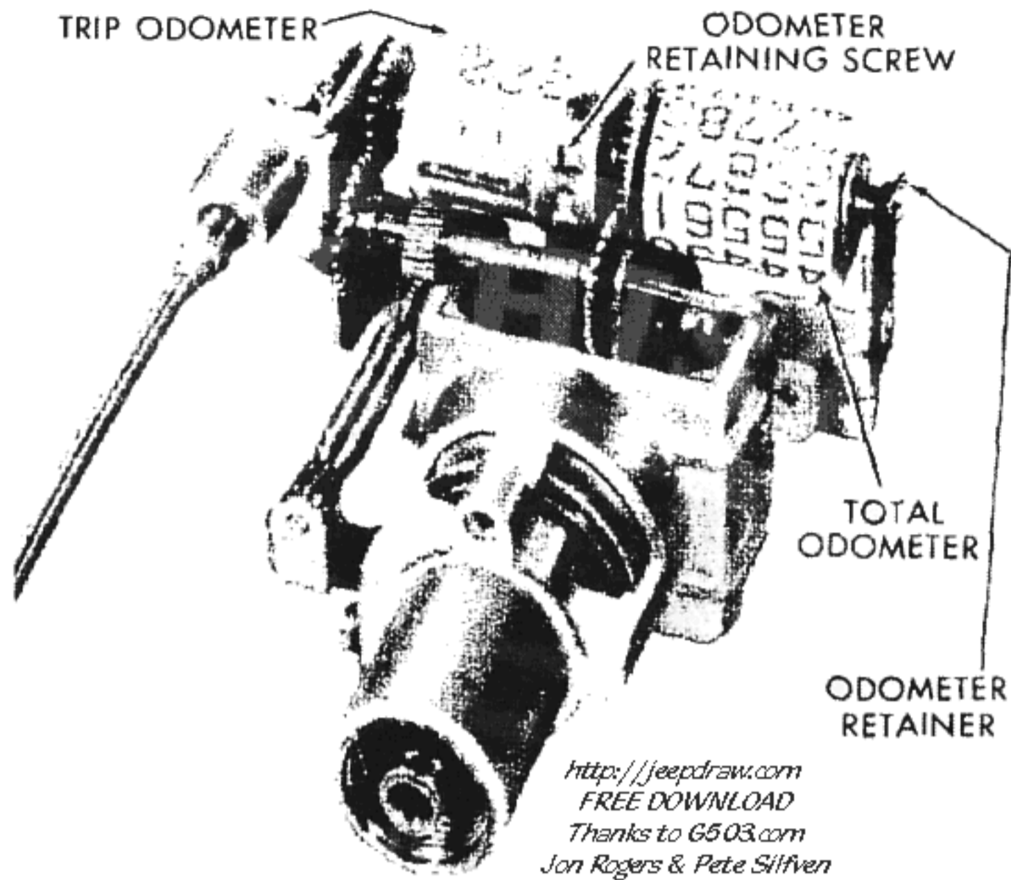
Figure 55—Speedometer Mechanism with Odometers in Line
