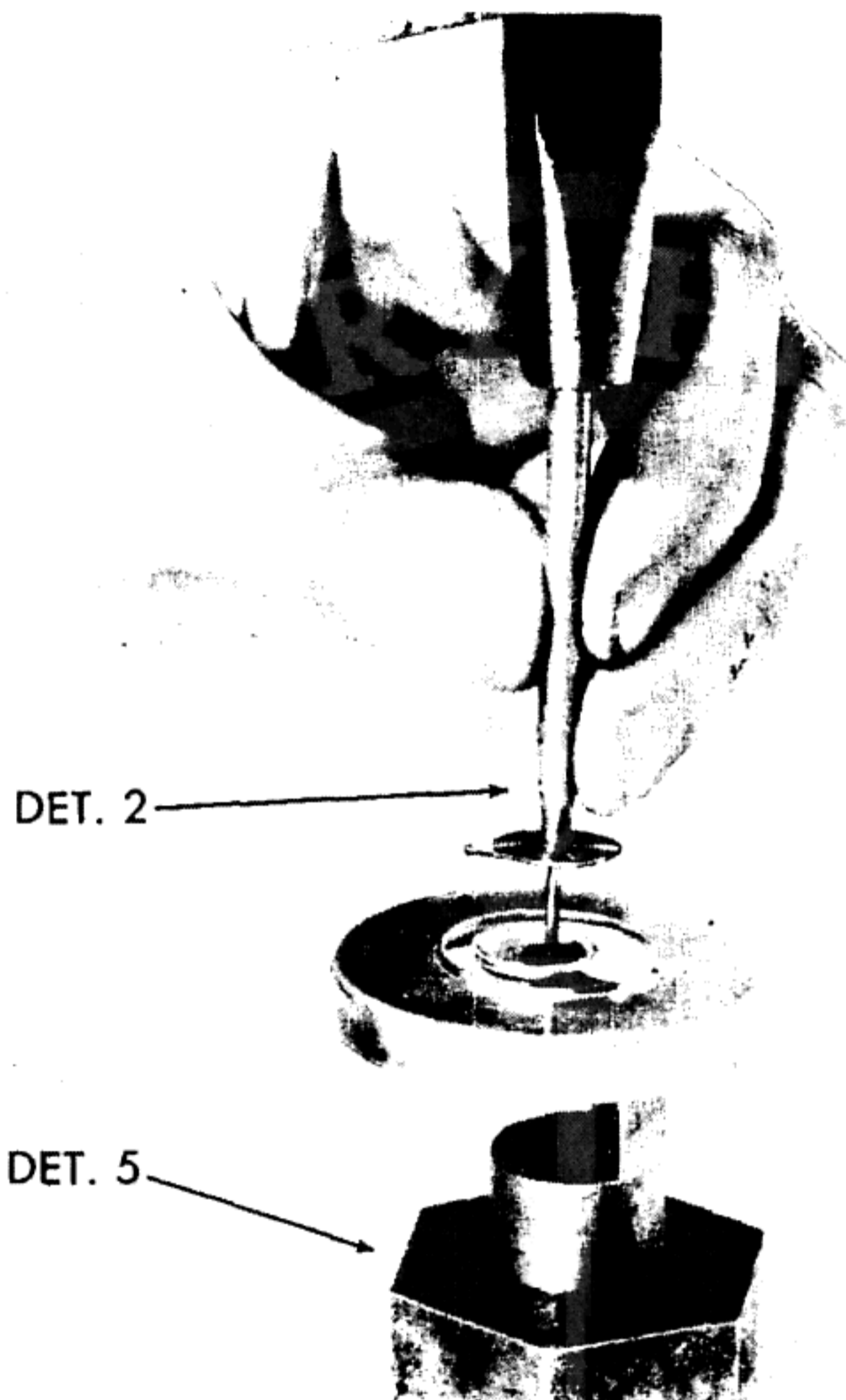
Figure 95—Replacing Hair Spring, Using Assembly Kit (T-29)
