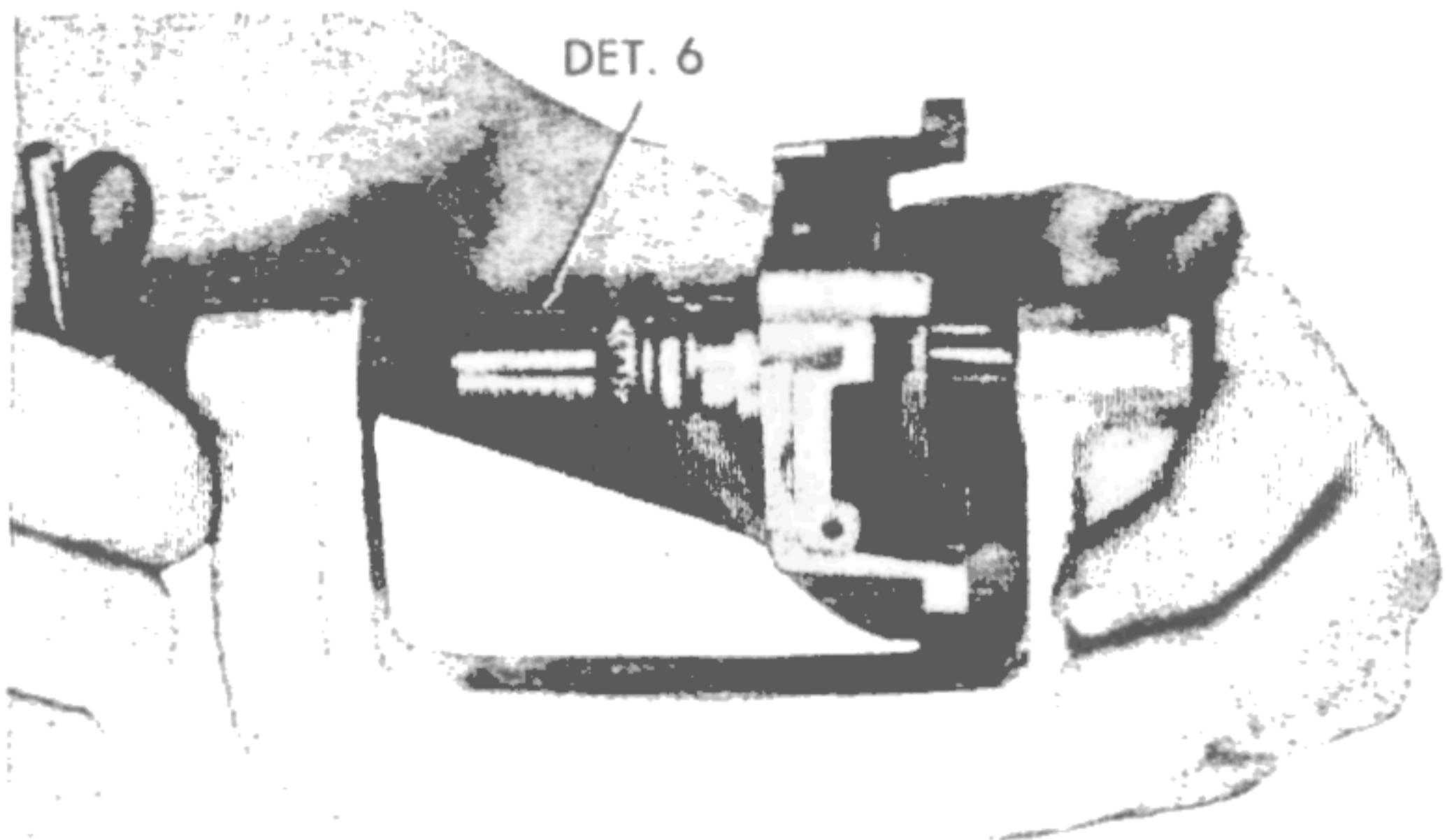
Figure 92—Flaring Magnet Shaft, Using Fixture (T-170666 with Det 6)
