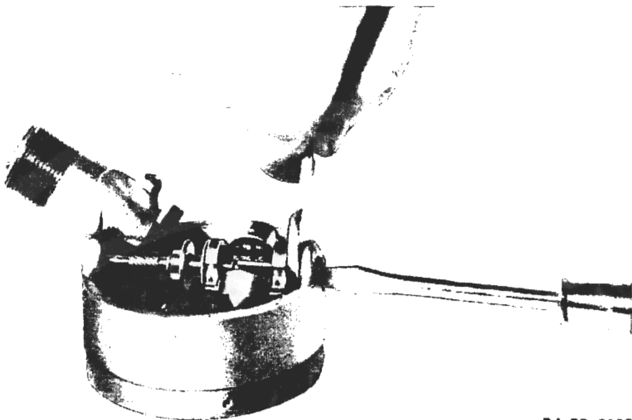
Figure 108—Loosening Upper Ball Race Lock Nut
