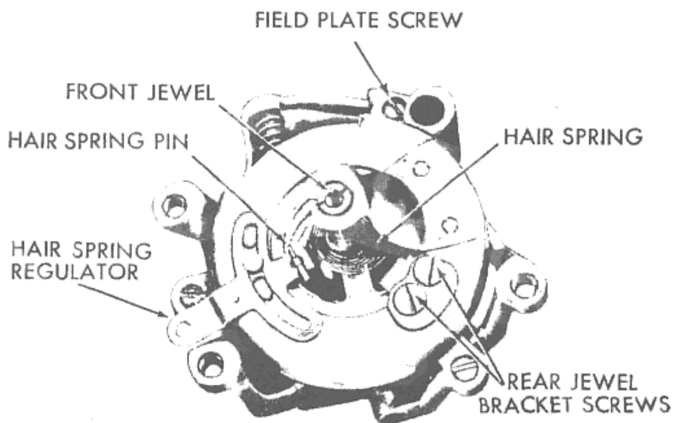
Figure 83—Speedometer Mechanism (Odometer Frame Removed)
