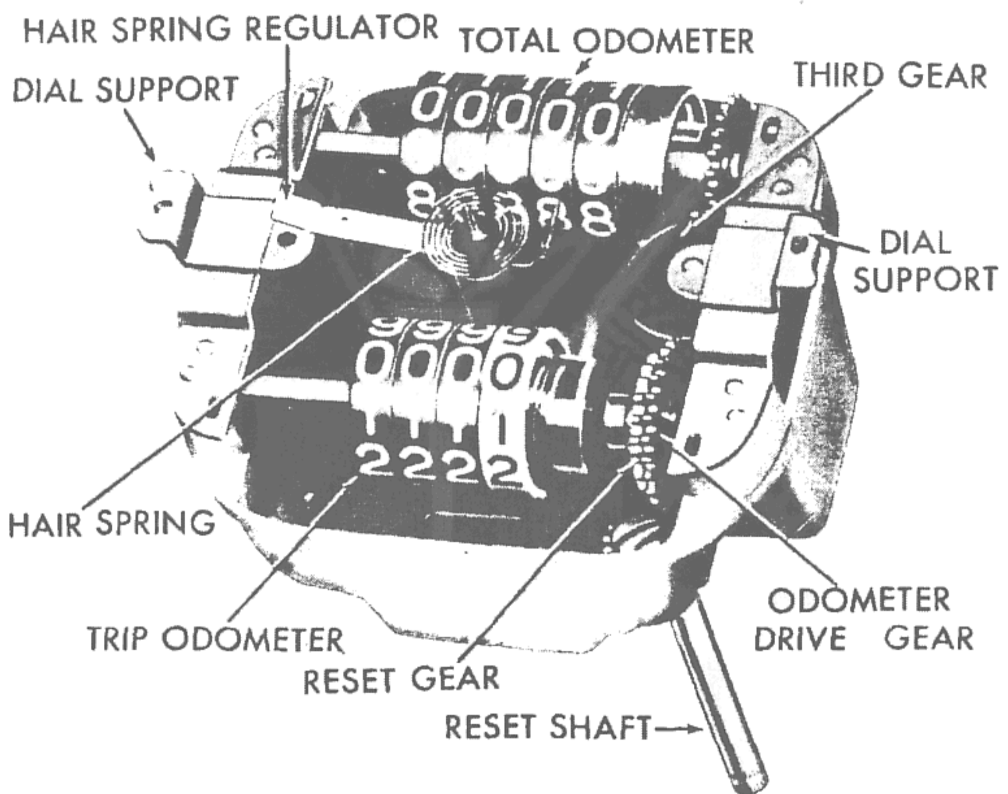
Figure 114—Speedometer Mechanism (Dial Removed)
