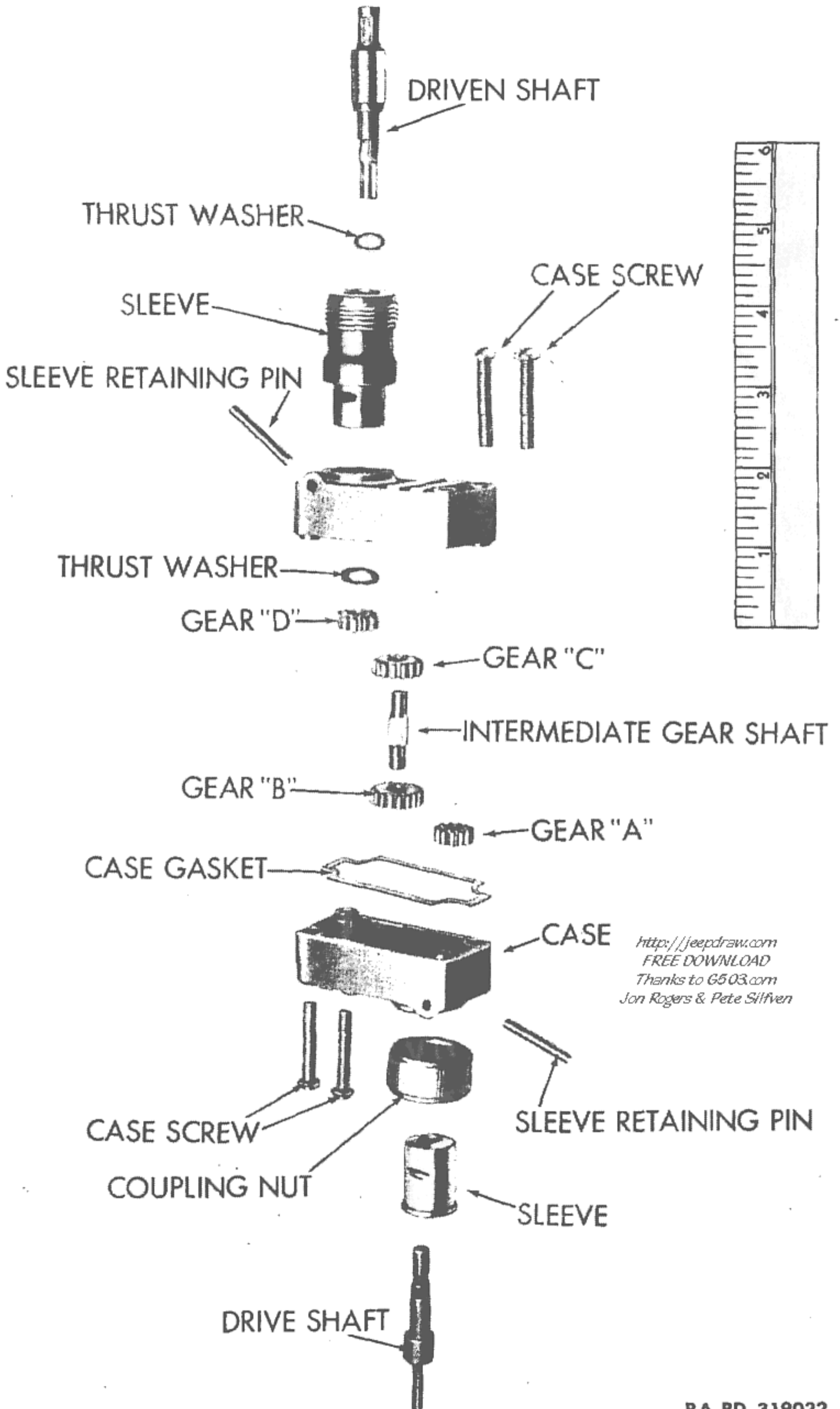
Figure 137—Stewart-Warner Type 666 Drive Joint, Disassembled
