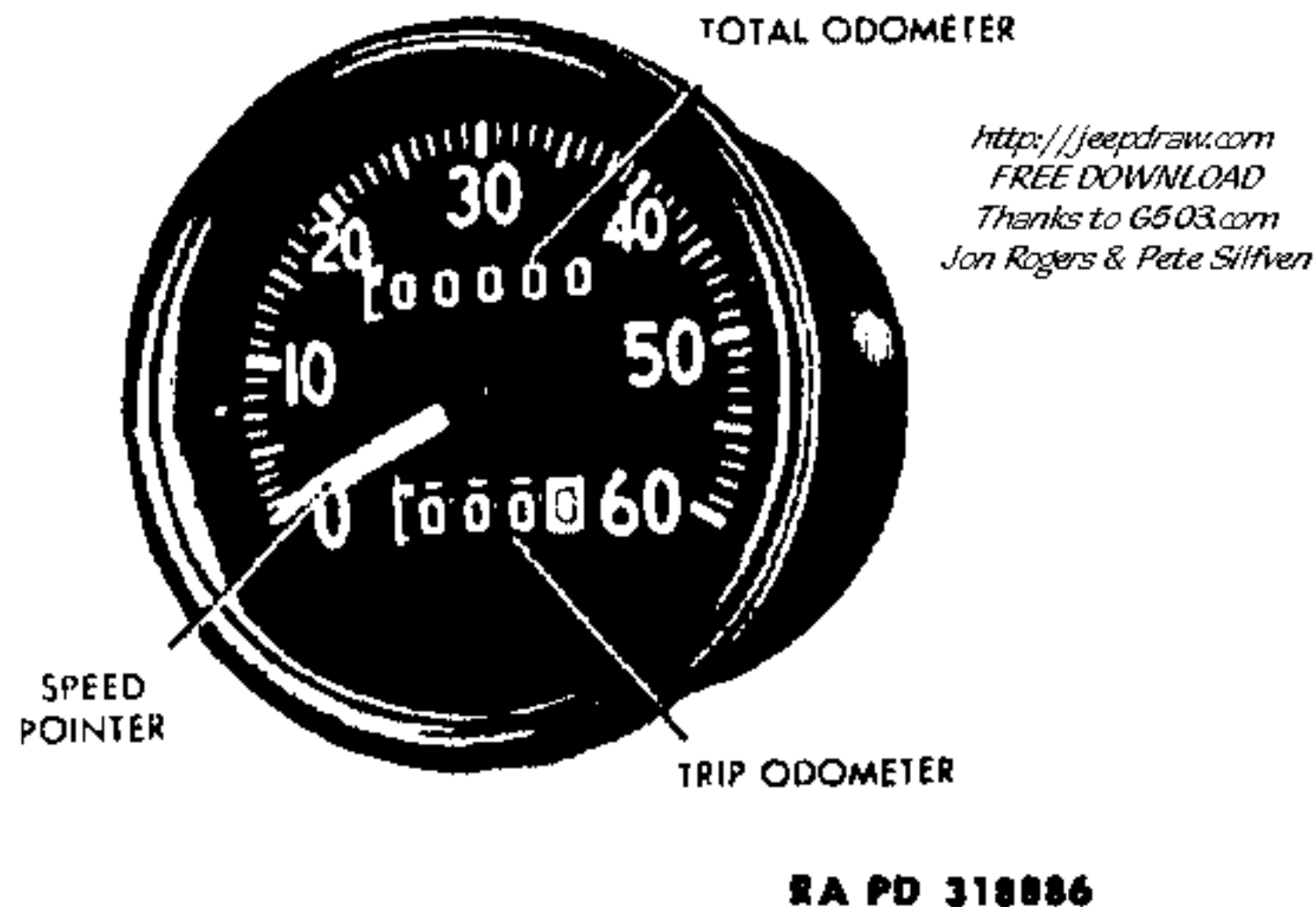
Figure 1—Speedometer
