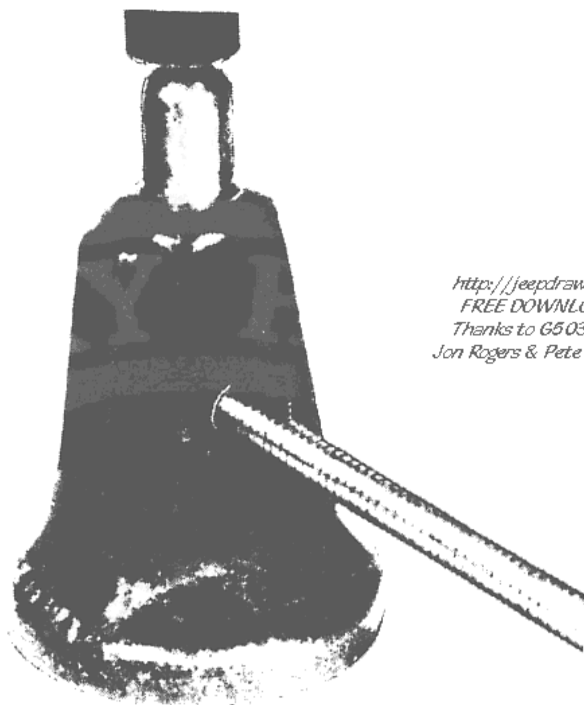
Figure 130—Crimping Ferrule, Using Fixture (T-52644)
